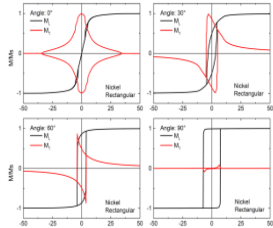
Fig. 5. Longitudinal and transversal hysteresis loops, simulated for the rectangular hexagon prepared from nickel.
